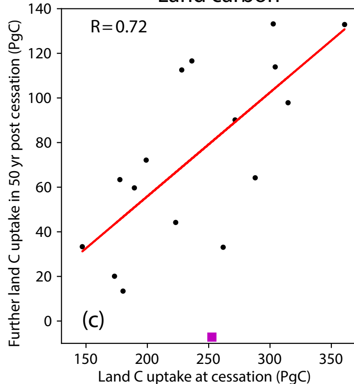
Land carbon
