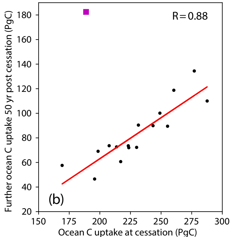
Ocean carbon
