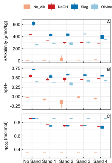
Figure 3. Results of Experiment 1. Changes of (A) alkalinity and (B) \text{pH}_T from the beginning to the end of the 6.8 days experiment. (C) \eta_{\text{CO}_2} at the end of the experiment. Boxplots are based on three replicates per treatment. Colours refer to the added alkalinity source (No_Alk means no alkalinity source was added). The alignment on the x-Axis indicates if or which sand sample was present in the incubation bottles (“No Sand” means no Sand was added).
