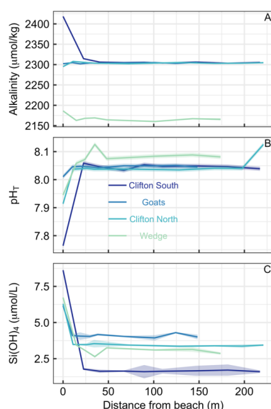
Figure 2. Transects of (A) alkalinity, (B) \text{pH}_T , and (C) \text{Si(OH)}_4 at four different beach locations in southern Tasmania (see Table S1 and Fig. S1 for locations). The first sampling was at the upper end of the swash zone and then 7-8 more samples were taken until 150-200 m offshore. Lines and shaded areas show averages and uncertainties, respectively.
