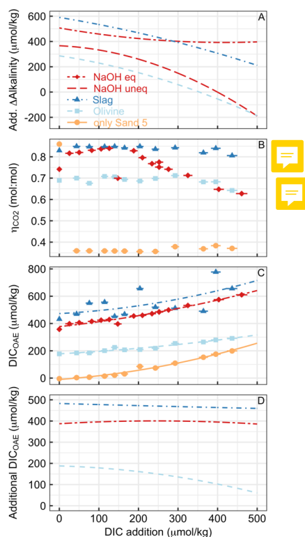
Figure 7. Various measures of OAE efficiency under increasing additions of DIC (DIC could for example be CO 2 from the respiration of organic material in sediments). (A) The additionality of ΔAlkalinity. (B) η CO2 at the end of the experiment. (C) DIC OAE , i.e., how much seawater CO 2 could have potentially been absorbed with the amount of ΔAlkalinity provided by the various alkalinity sources. (D) The additionality of DIC OAE . Please note that panels (B-D) only show data for the equilibrated NaOH scenario. I omitted the unequilibrated scenario for logical reasons, i.e., because the core assumption in this scenario (no CO 2 equilibration with the atmosphere after OAE) is at odds with the necessary assumption of CO 2 equilibration to calculate η CO2 (see eq. 10).
