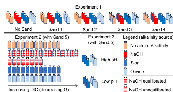
Figure 1. Design of Experiments 1, 2, and 3. Bottles represent treatments with incubation of seawater, sand, and alkalinity sources (color code represents alkalinity source). In Experiment 2, NaOH was used as alkalinity source in two explicit scenarios as described in section 2.2.2.
